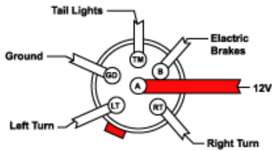
7-Way Car End
