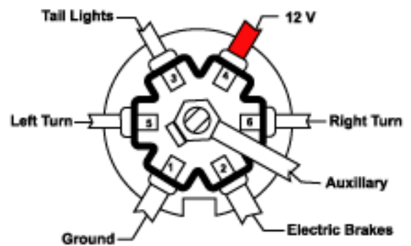
7-Way Trailer End
