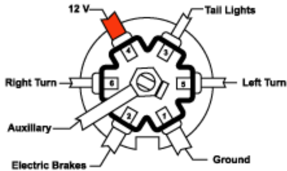
7-Way Car End
